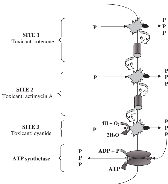
Figure 10.7 Electron ( e^- ) transport along the inner mitochondrial membrane resulting in the pumping of protons (P) out of the mitochondrial matrix. Protons are shuttled back into the matrix through the ATP synthetase complex where ATP is generated. Sites of toxicant action are indicated.
